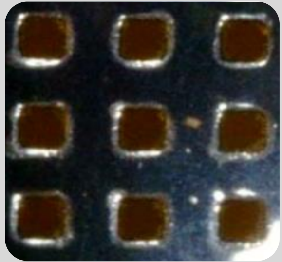
NanoClear ® Treated Stencil after 40 prints
