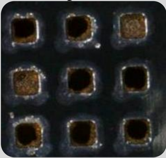
Untreated Stencil after 14 prints
